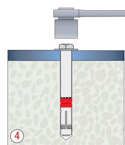
4 Tighten Bolt to Recommended Torque
